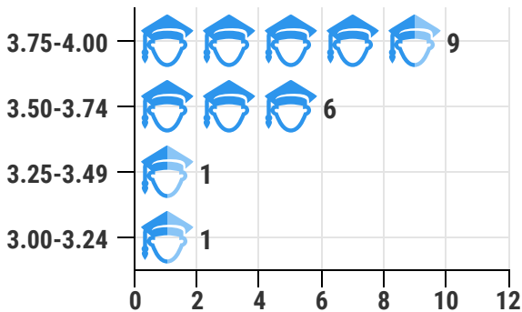
GPA Distribution
